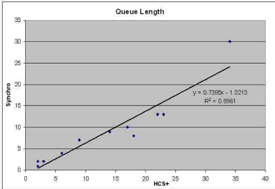
Figure 5-1: Comparison of Queue Lengths Estimated by HCS+ and Synchro.
